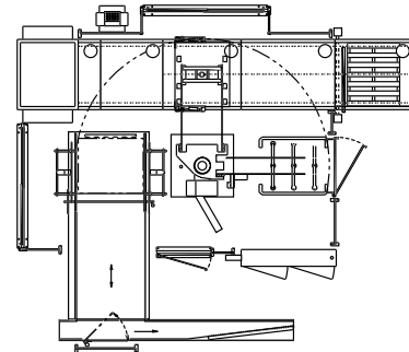
FULLY AUTOMATIC PALLETIZER/DEPALLETIZER
