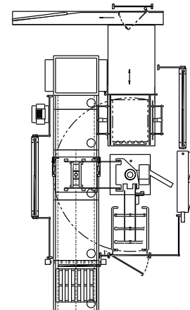
FULLY AUTOMATIC PALLETIZER/DEPALLETIZER
