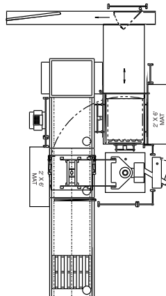
SEMI-AUTOMATIC PALLETIZER/DEPALLETIZER WITH FULLY AUTOMATIC PALLET HANDLING
