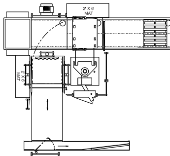
SEMI-AUTOMATIC PALLETIZER/DEPALLETIZER WITH FULLY AUTOMATIC PALLET HANDLING
