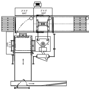
SEMI-AUTOMATIC PALLETIZER/DEPALLETIZER
